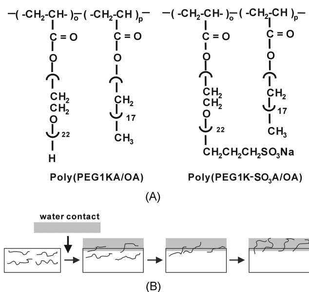
Fig. 1. (a) Structures of the synthesized copolymers. (b) Schematic diagram of self-transformable device with time course. After contacting with water, hydrophilic block starts to re-orient from arbitrary conformation towards water phase, whereas hydrophobic block is to be anchored in membrane matrix by hydrophobic force.
